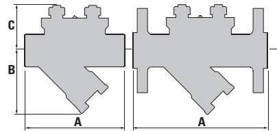
Clearance for Strainer Removal: HPTD 5 in (127 mm) min.
